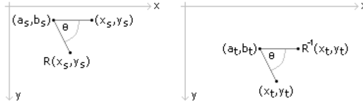
Figure 1. Left: The original and rotated points in the source block. Right: The rotated point in the target block.
